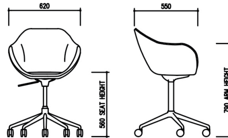
TUB High Height Adjustable
