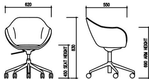
TUB High Height Adjustable
