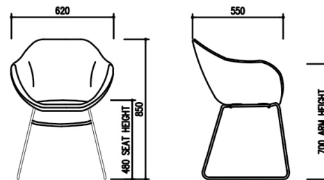
TUB High Sled
