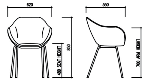
TUB High Metal 4 Leg
