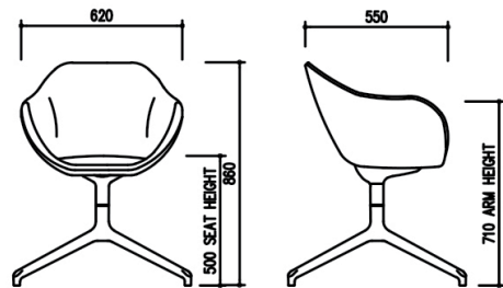
TUB High 4 Star Glides
