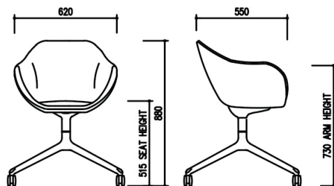
TUB High Castors
