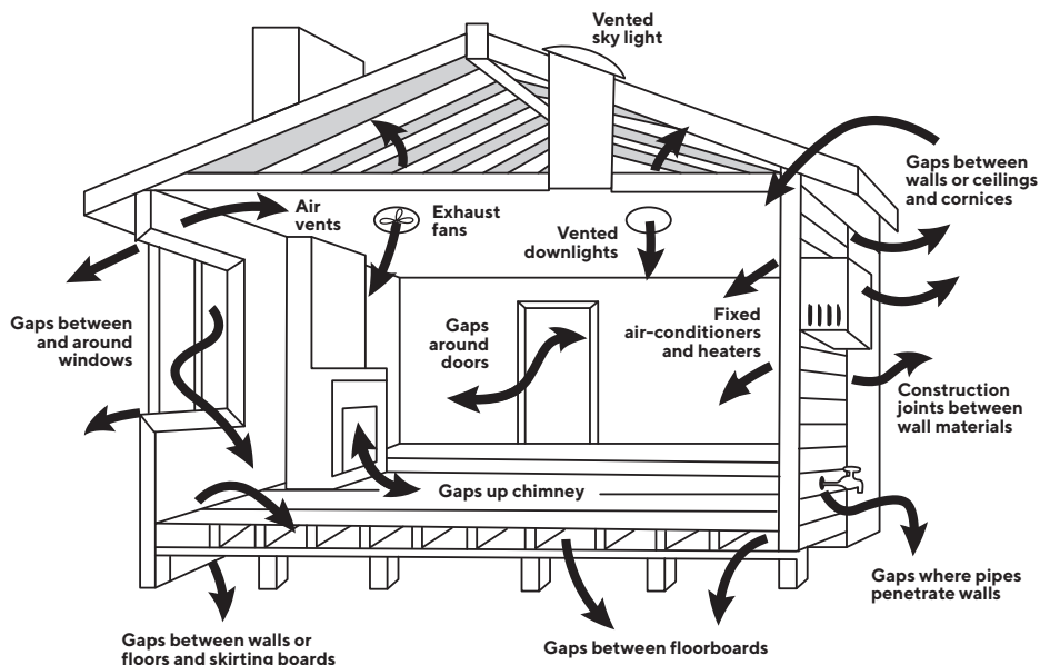
Common air leakage points
